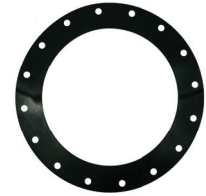
500mm - 16 HOLES
